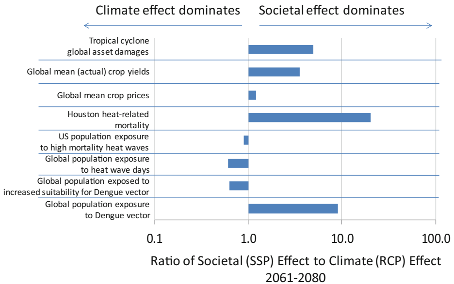
Fig. 3 Ratio of the difference in impact outcomes due to alternative climate change scenarios (RCP4.5 vs RCP8.5) and the difference due to alternative socioeconomic development pathways (SSP3 vs SSP5). Results from Gettelman et al. (2017), Ren et al. (2016), Marsha et al. (2016), Anderson et al. (2016b), Jones et al. (submitted), and Monaghan et al. (2015). Tropical cyclone damage results based on comparison of impacts in SSP-only and climate-only scenarios compared to present
