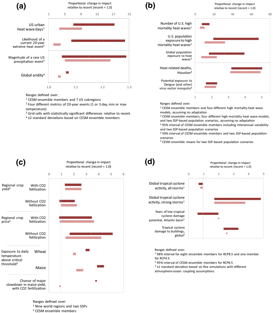
Fig. 1 Differences between RCP8.5 and RCP4.5 for impacts related to a extreme events, b health, c agriculture, and d tropical cyclones (see Fig. S2 for additional results related to extreme events and agriculture). Bars show uncertainty ranges for impacts in RCP8.5 (red) and RCP4.5 (pink) for the late twenty-first century relative to a recent period (2061–2080 relative to 1986–2005 unless otherwise indicated). Outcomes are expressed as the ratio of impacts relative to recent (where recent = 1.0). For societal impacts, total impacts are shown, i.e., the impact due to both climate and societal change. Ranges are defined differently for each impact (see Table S2 and notes to each panel); they are comparable between RCPs for a given impact but not across impacts. Note that a and b employ two different x -axis scales; the area above/below the horizontal dividing line corresponds to the axis at the top/bottom of the figure
