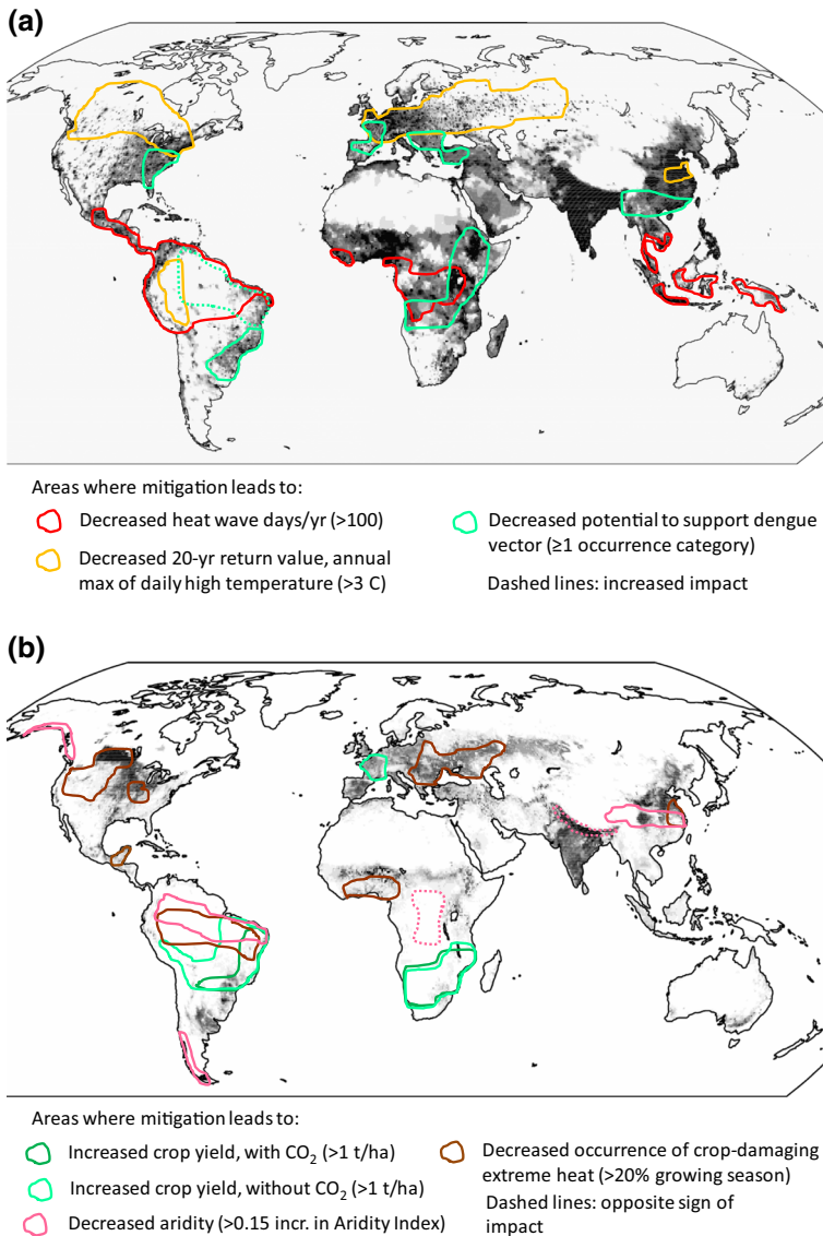
Fig. 2 a Spatial distribution of especially large benefits of mitigating from RCP8.5 to RCP4.5 superimposed on the spatial distribution of the projected population in 2070 for SSP5. Results from Jones et al. (submitted), Tebaldi and Wehner (2016), and Monaghan et al. (2015). b Same as a , but superimposed on the spatial distribution of the projected cropland in 2070 for SSP5, with results from Ren et al. (2016), Levis et al. (2016), Tebaldi and Lobell (2015), and Lin et al. (2015). See Fig. S3 (SM) for maps of benefits from individual impacts
